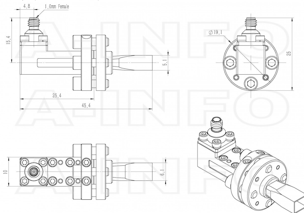
1.0mm-Female Output (P/N: LB-12-10-C-1.0F)
